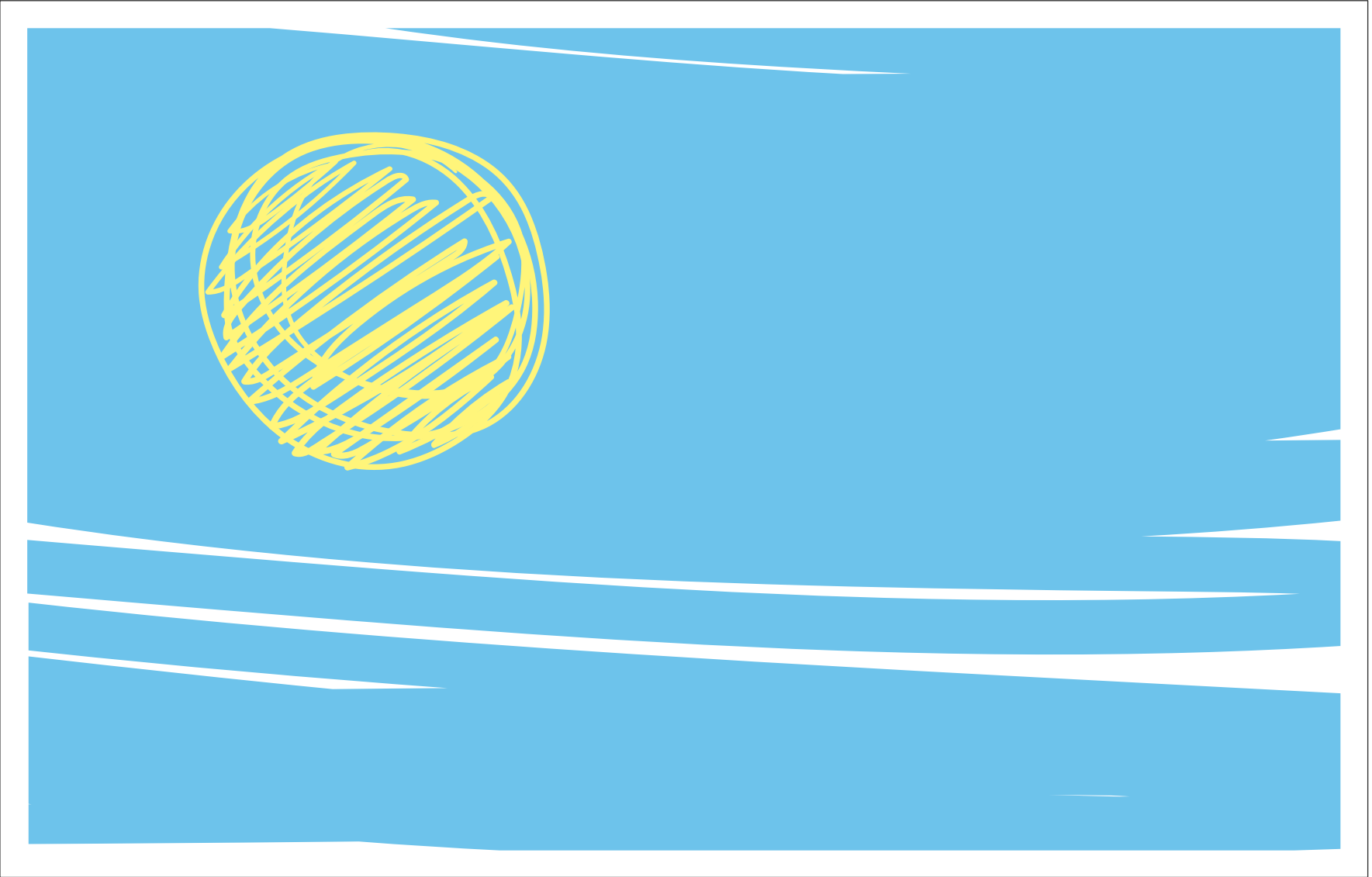
Figure 4.1: Minilesson Object
